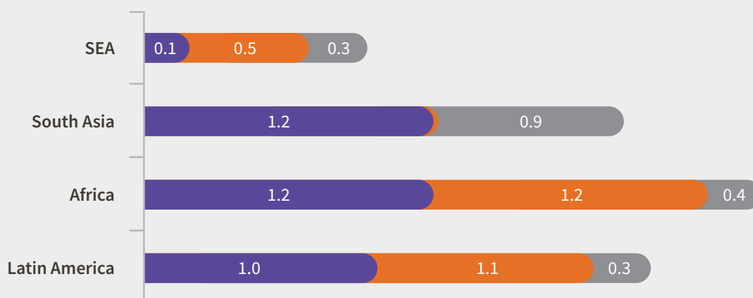
Figure 4: LMIC region wise GHG emission data across three stages of the agri supply chain (Total ~8.2 GtCO 2 e q )
